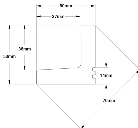
Polyurethane Coving
