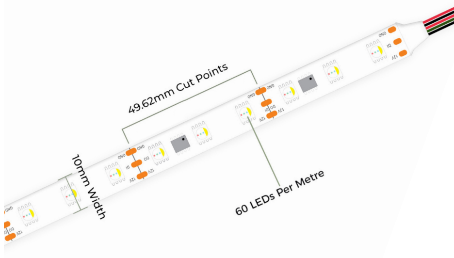
TAPE DIAGRAM
