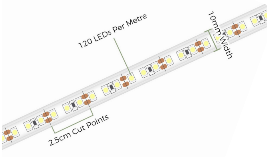
TAPE DIAGRAM
