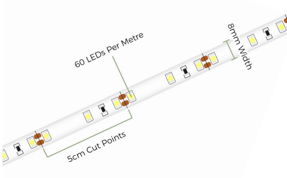
TAPE DIAGRAM
